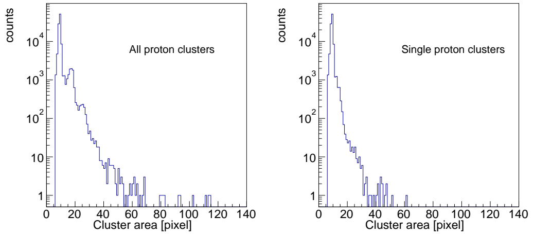
Figure 3.19: Left: The distribution of cluster area for all proton clusters with area \geq 6 . The local maxima appearing in the distribution correspond to the cases of one proton hit or several merged nearby proton hits. Right: The distribution of cluster area for the single proton clusters with area \geq 6 . Note that the peaks corresponding to merged nearby proton hits are largely suppressed. The distributions correspond to the case without any plates in the energy degrader.
